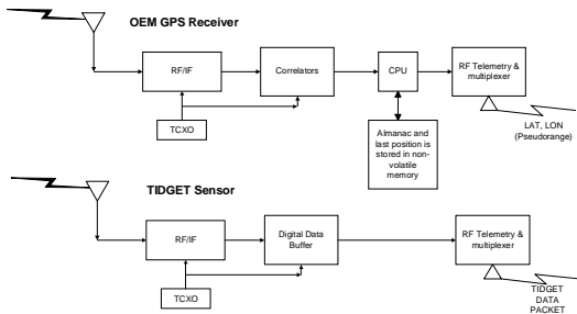
Figure 2 TIDGET Sensor
