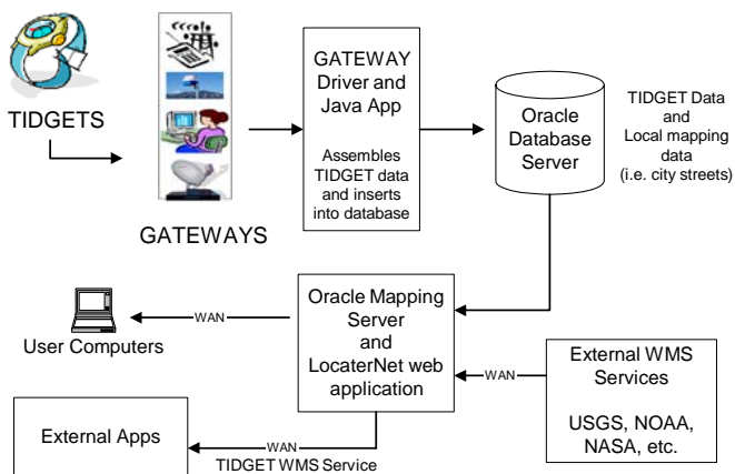
Figure 9 LocatorNet LBS Architecture
