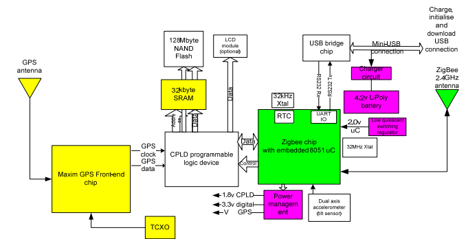
Figure 5 TIDGET/ZigBee Device Components
