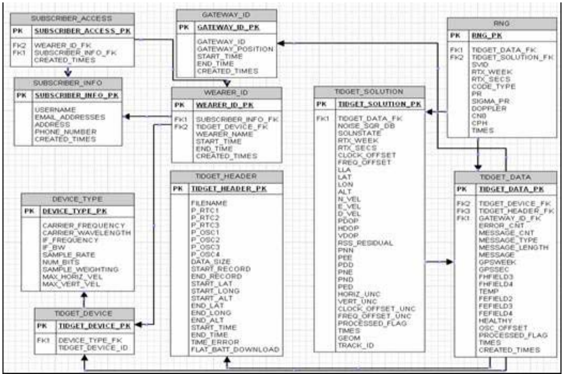
Figure 8 Portal Database Schema
