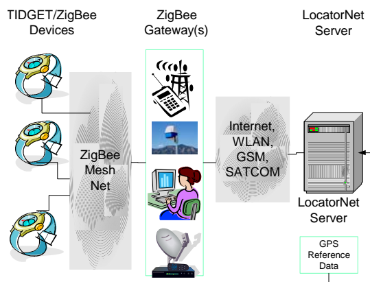
Figure 1 LocatorNet System Architecture
