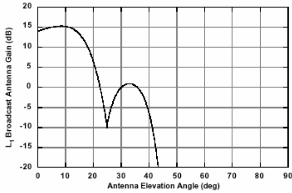
Figure 7 GPS II/II-A Gain Pattern
