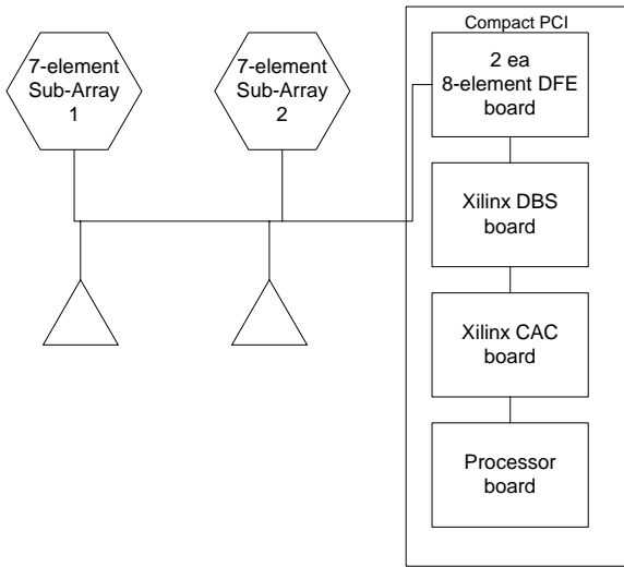
Figure 1 SSGR Design
