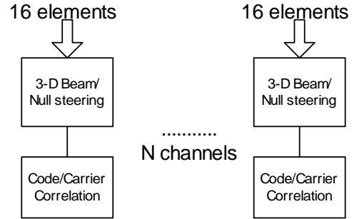
Figure 3 Digital Beam/Null-Steering Firmware Functions
