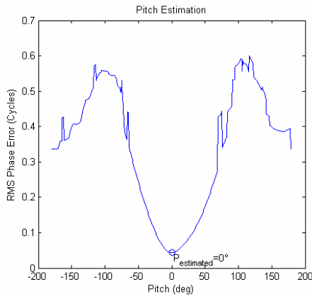
Figure 11 Pitch Estimation
