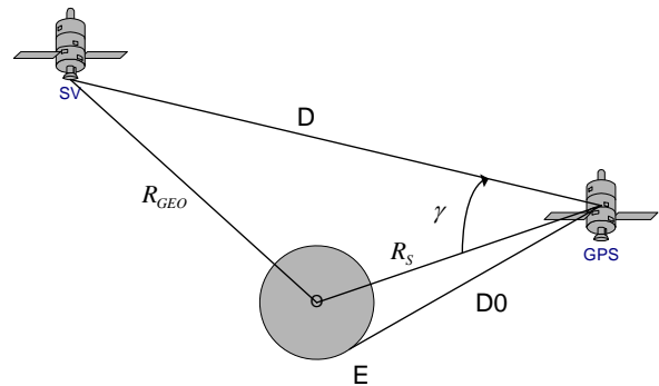
Figure 6 GPS-to-Spacecraft Geometry
