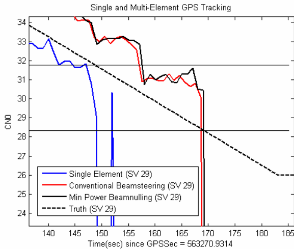
Figure 15 Low Power Tracking Results (Detail)
