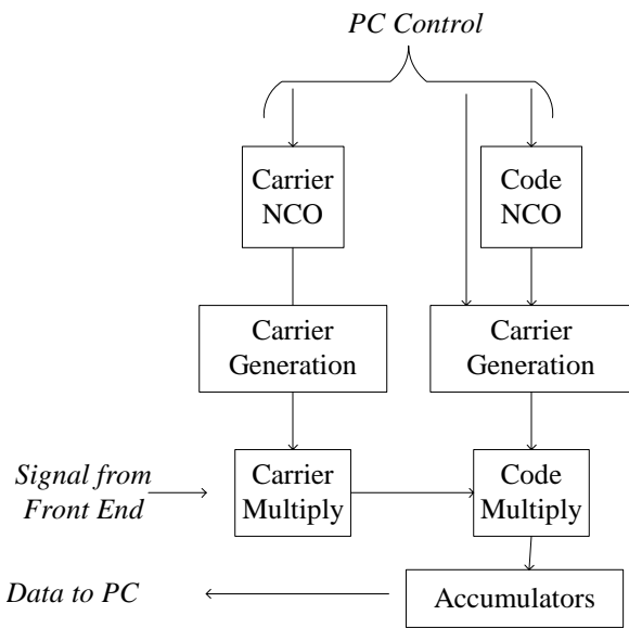
Figure 4 Correlator Functions
