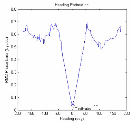
Figure 13 Heading Estimation
