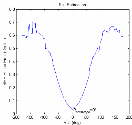
Figure 12 Roll Estimation
