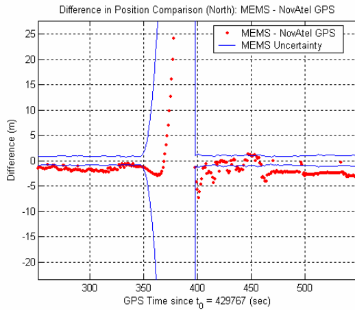
Figure 14 MEMS Inertial Navigation Results
