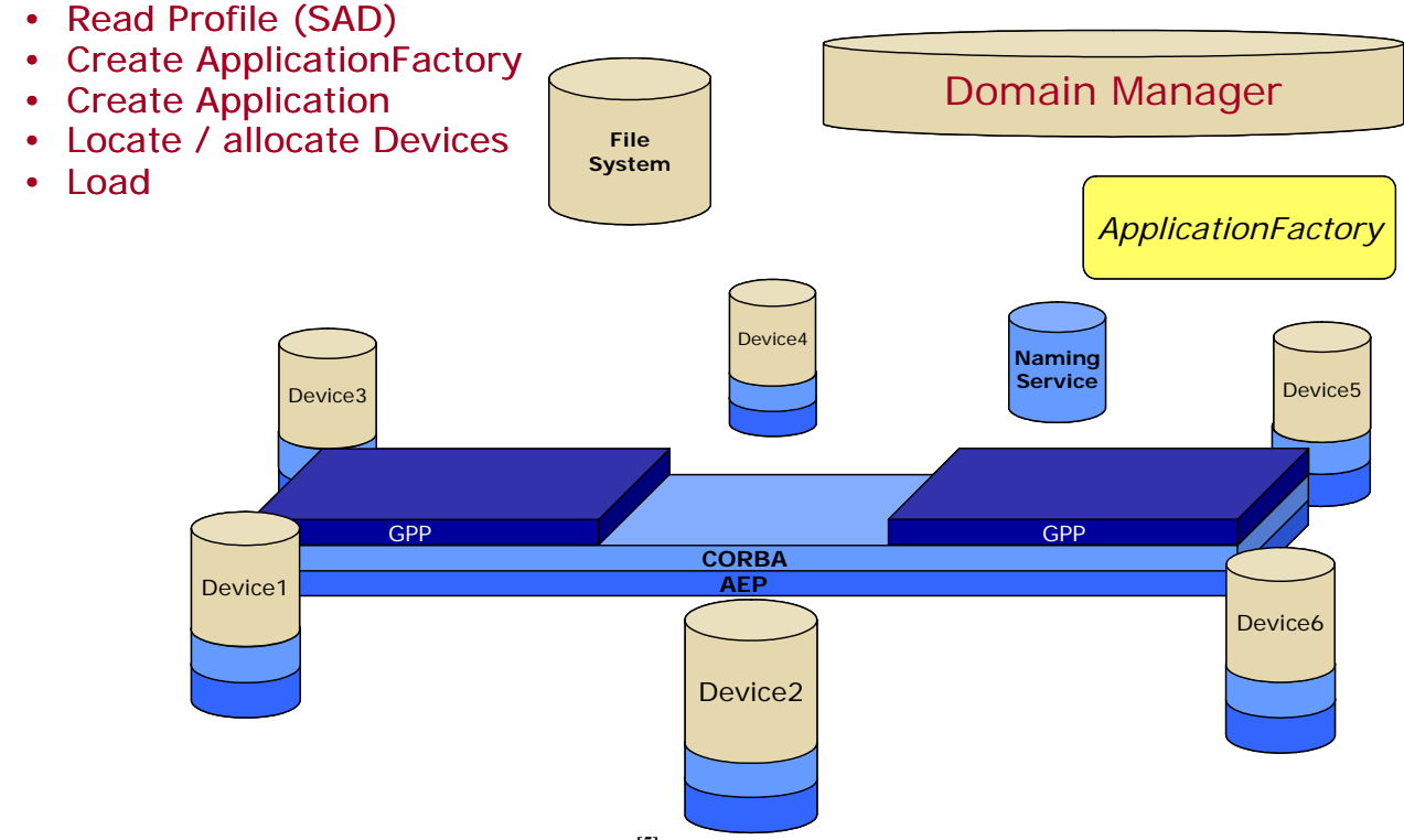
Figure 6 Waveform Instantiation and Deployment [5]
